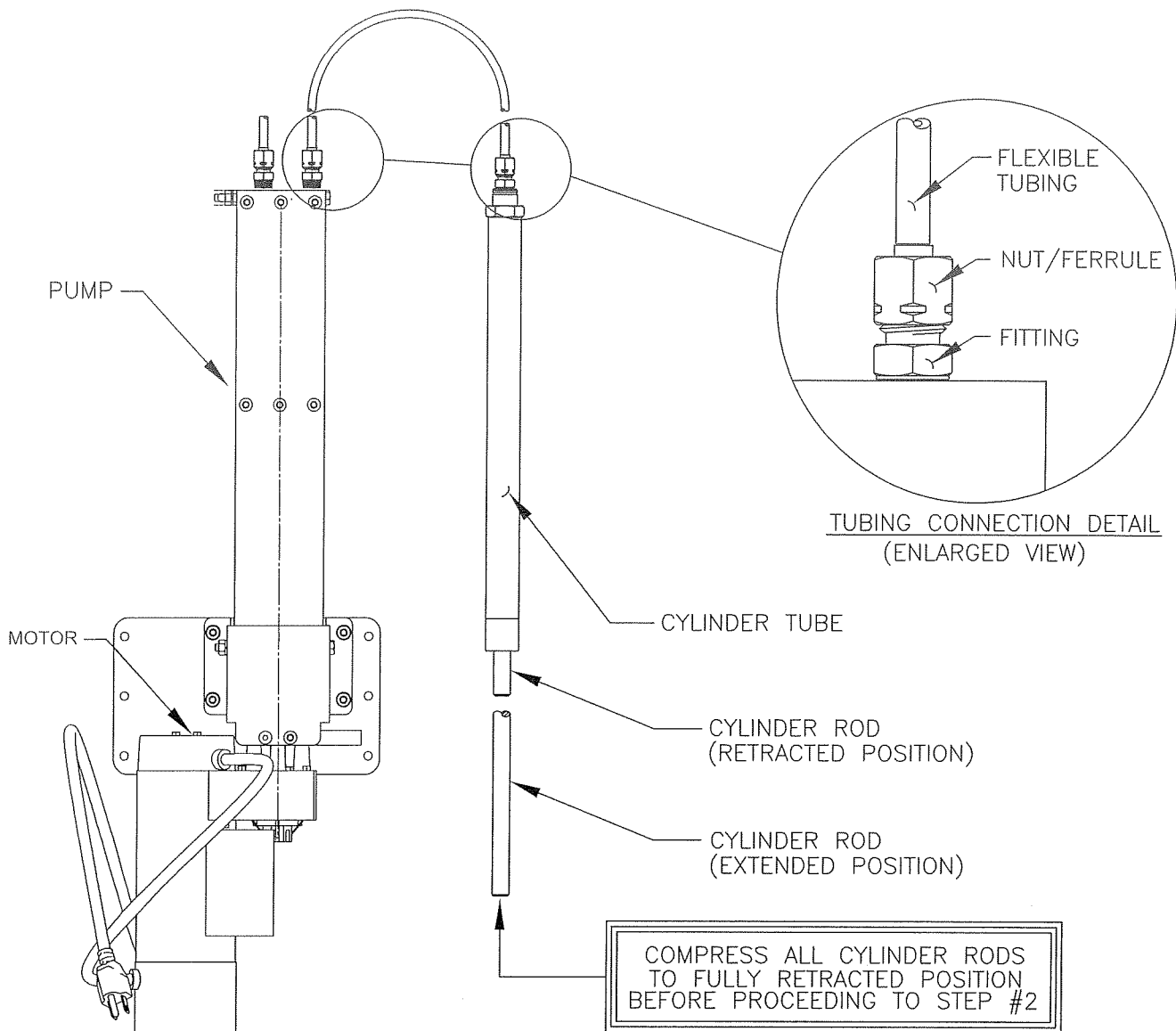
FIGURE 1 – ASSEMBLED SYSTEM
